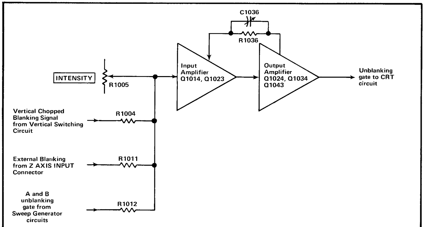
Fig. 3-15. Z Axis Amplifier detailed block diagram.
