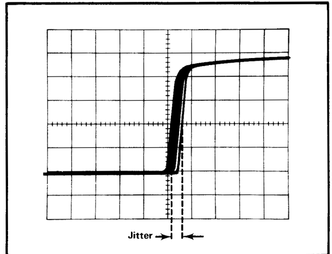
Fig. 2-25. Measuring pulse jitter.
