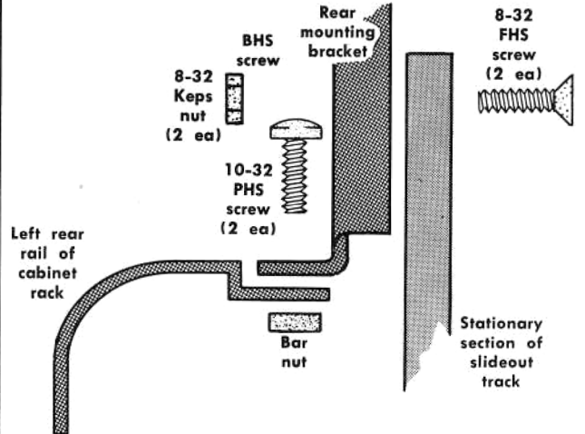
(B) Untapped rear rail
