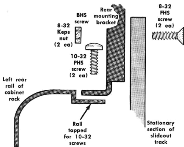
(A) Rear rail tapped for 10-32 screws
