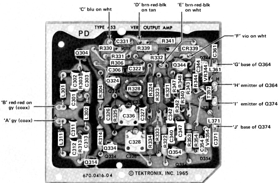
Fig. 8-4B. A-2. Vertical Output Amplifier circuit board.
