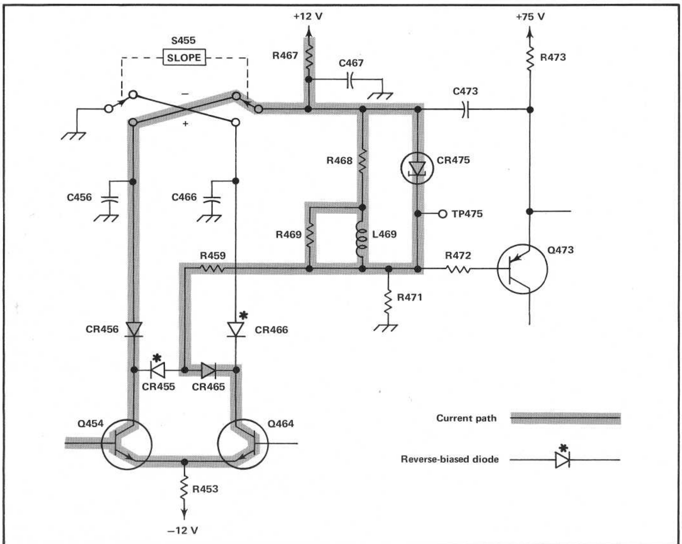
Fig. 3-9. Trigger path for negative-slope triggering (simplified A Trigger Generator diagram).
