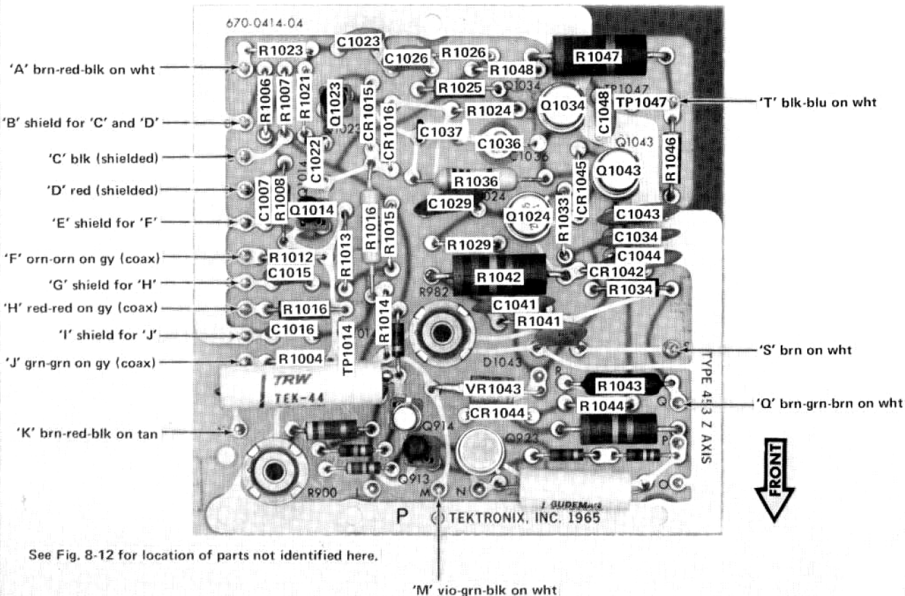
Fig. 8-11. P/O A5. Partial Z Axis circuit board.
