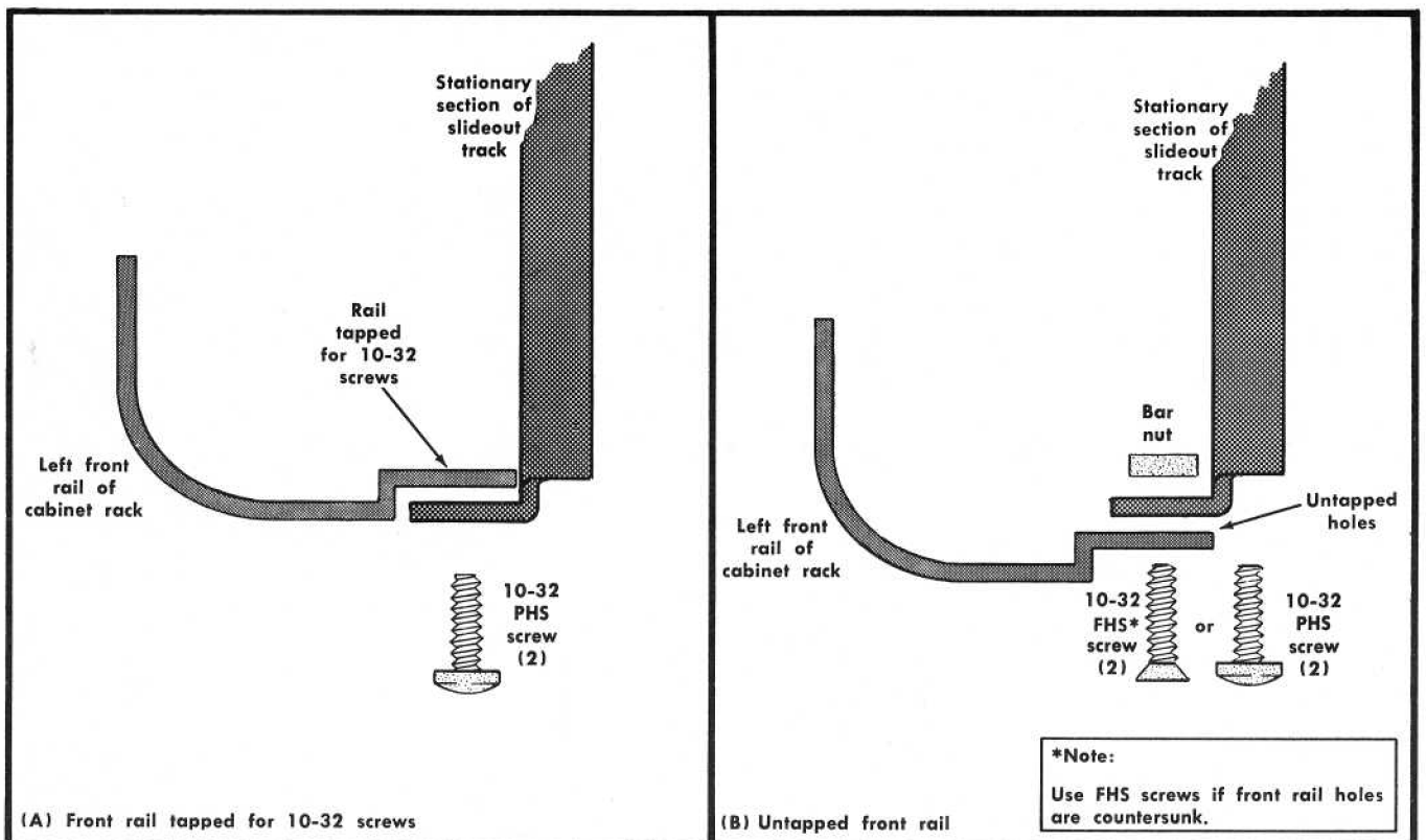
Fig. 6-4. Methods of mounting the stationary section to the front rails.
