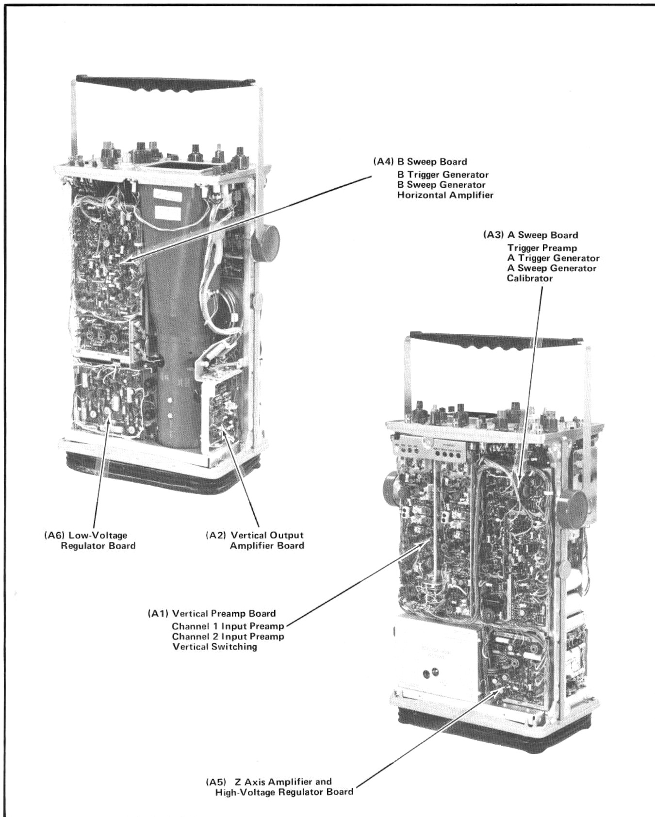
Fig. 4-4. Location of circuit boards in the 453A.
