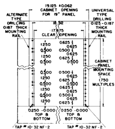
Fig. 6-11. Dimensional Drawing.
