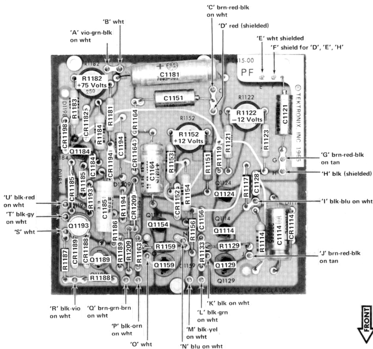
Fig. 8-13. A6. Low Voltage Regulator circuit board.
